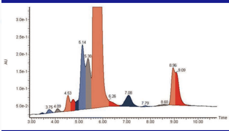
Expanded UPLC Chromatogram for Oligonucleotide Purity Analysis
